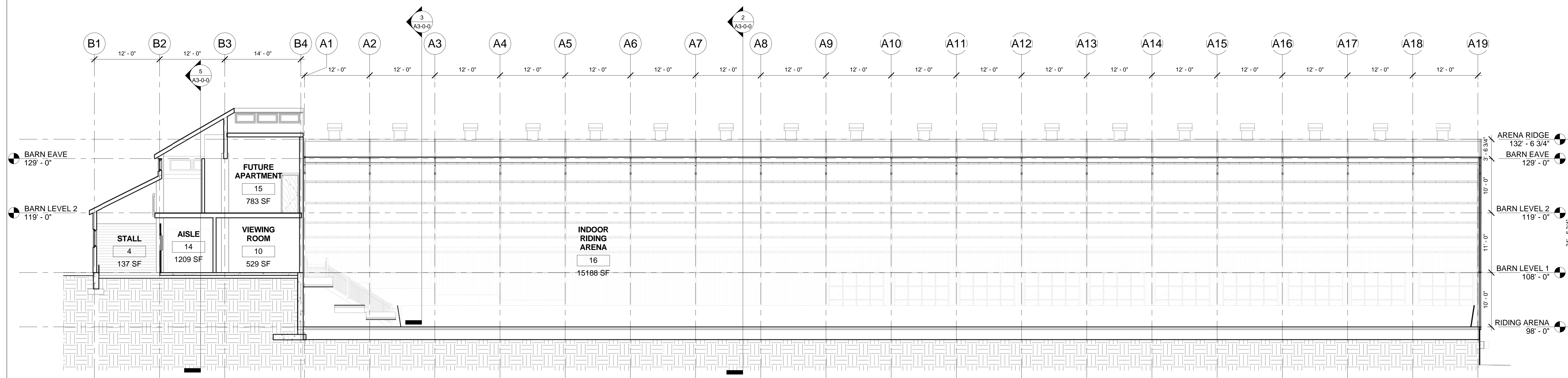
1 BUILDING SECTION 1 1/8" = 1'-0"
